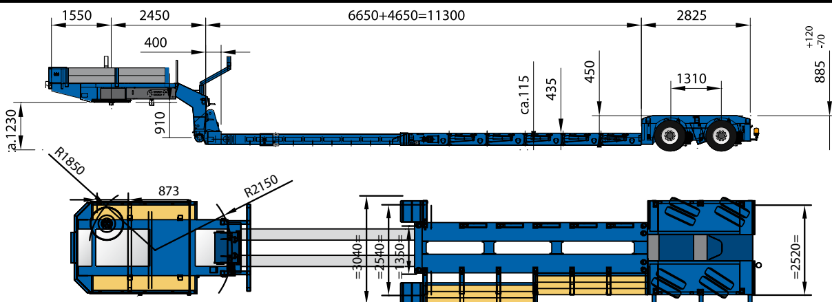
NOOTEBOOM EURO-38-02 LOW-LOADER
